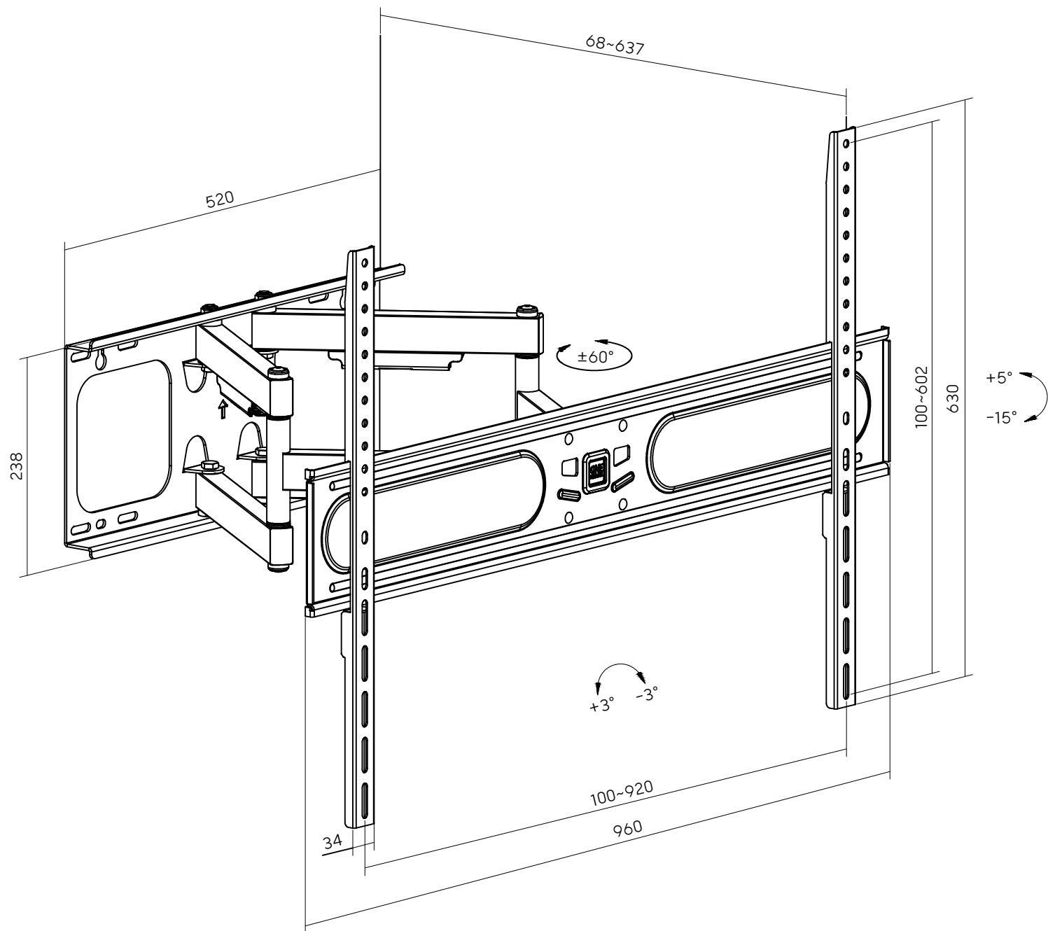
Dimensions (mm)
